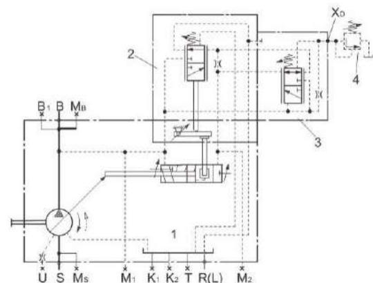
LR2G Schematic
