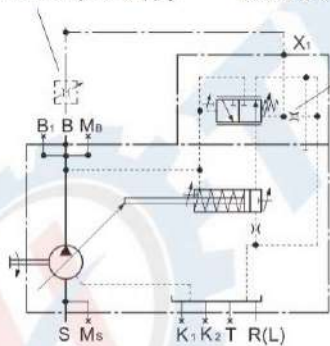
FR Schematic
