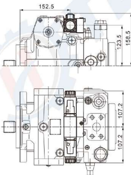
EP-Proportional control,electric
