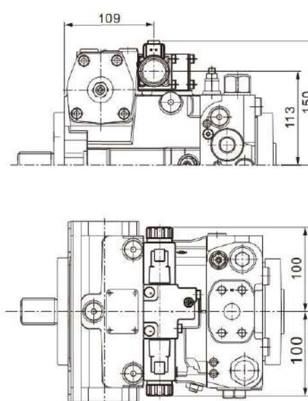
EZ-Two-point control,electric
