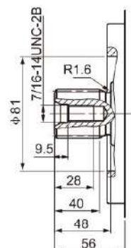
T spline shaft SAE J744 1 3/8in 21T 16/32DP 1)
