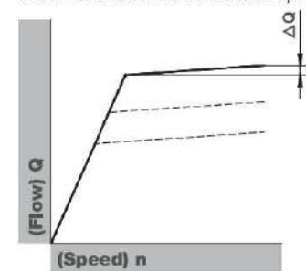
Static characteristic at variable speed
