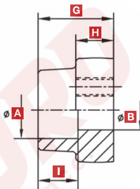
FLAT FACE Fig 2
