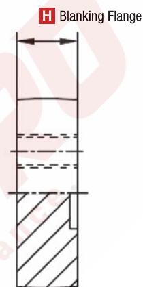
FLAT FACE Fig 2
