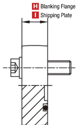
O-RING Fig 1
